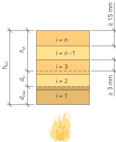
b) Residual cross-section h_{\text{ef, char}} layer d_{\text{char}} and non-load-bearing layer d_0 for single-sided fire exposure.
