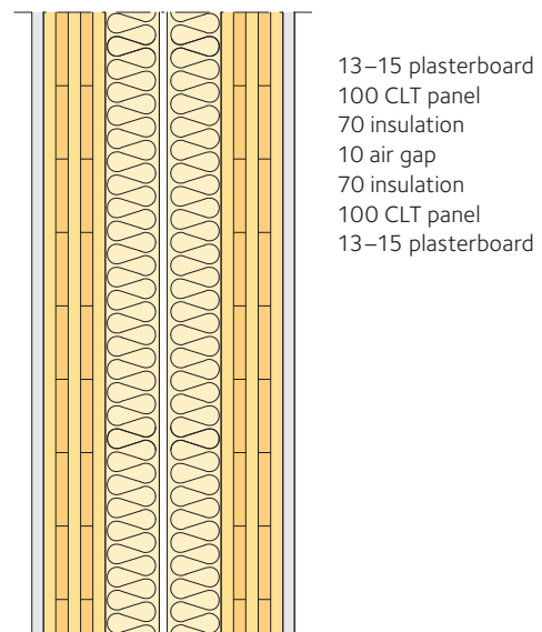
Figure 6.2 Example of partition wall between apartments using load-bearing CLT panel.
