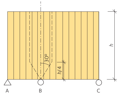
Figure 6.24 Load spread from support reaction.
