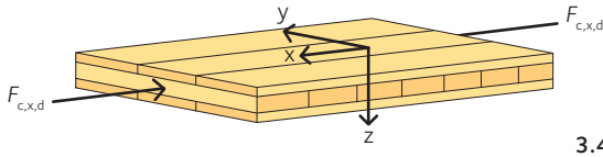
Figure 3.15 CLT panel with compressive force parallel with surface layer.
