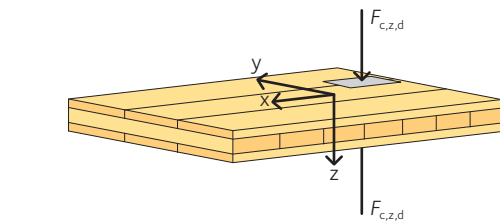
Figure 3.17 CLT panel with compression force perpendicular to its plane.
