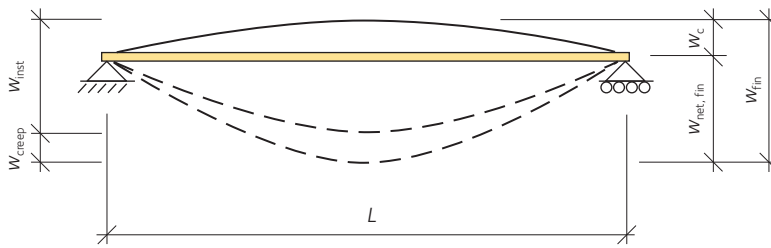
Figure 5.8 Definitions of deflection.
