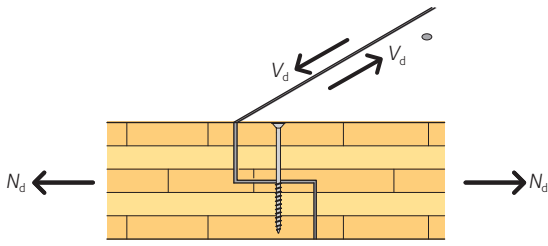
Figure 4.10 Half-lap joint.
