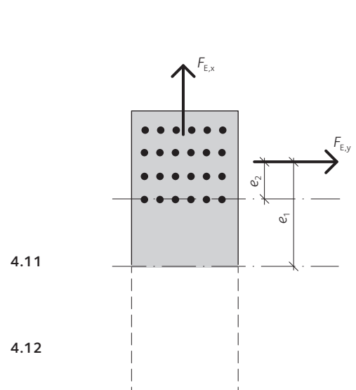
Figure 4.32 Connecting of CLT panel using steel plates. Schematic diagram. The plates can be fastened using nails or wood screws.
